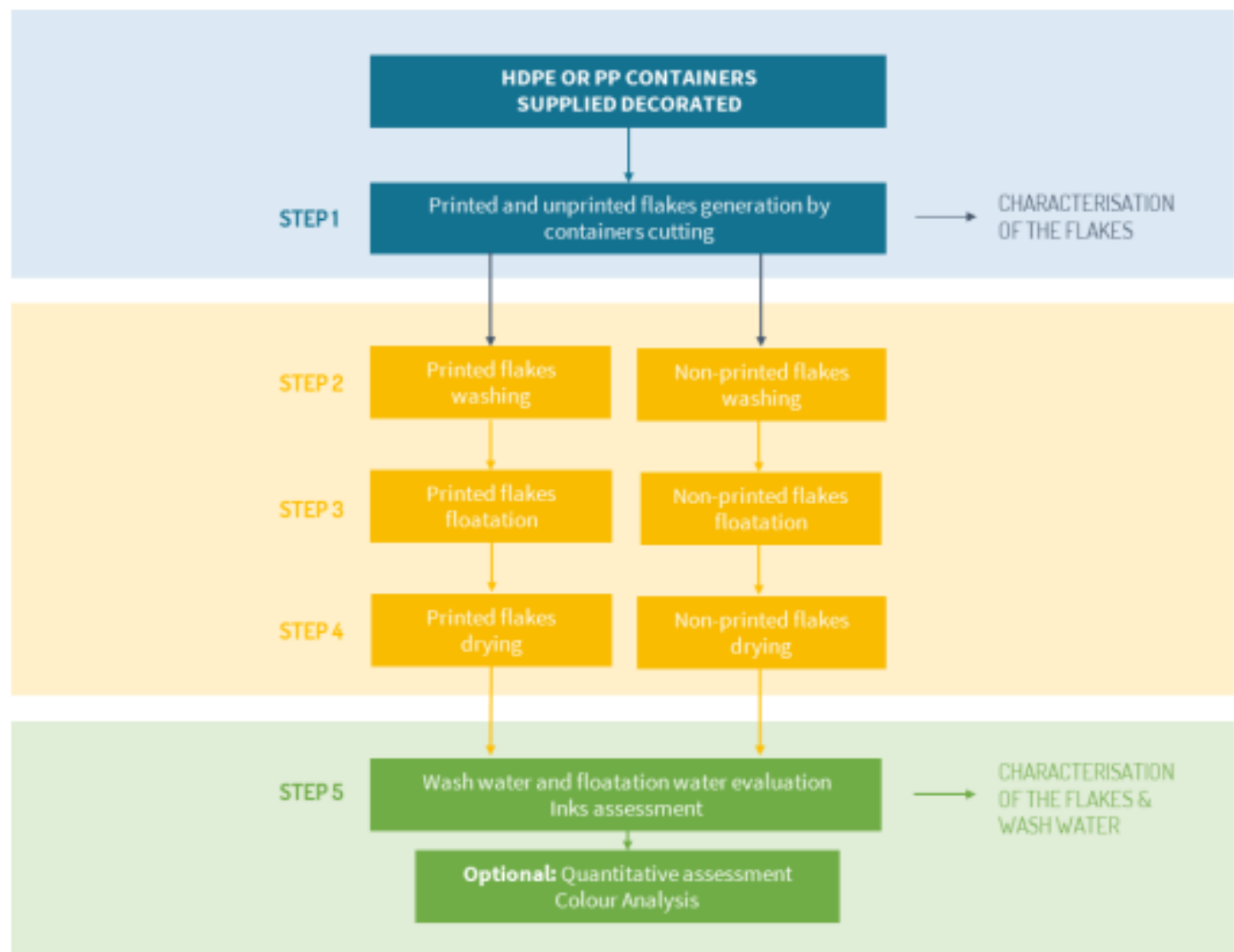
Figure1: Methodology Diagram
