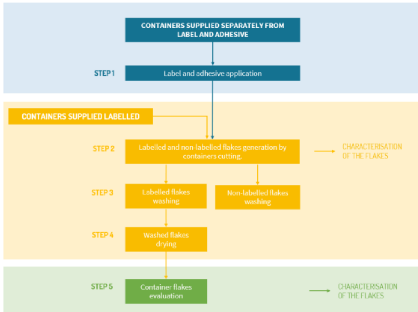
Figure1: Methodology Diagram
